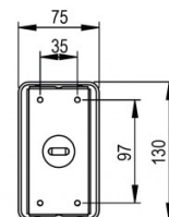
WALL BRACKET
