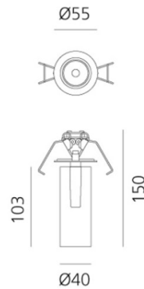
Vector Semirecessed 40
