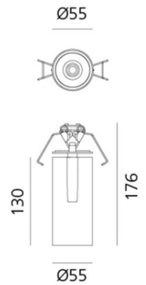
Vector Semirecessed 55
