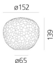
Meteorite 15
