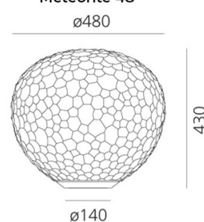
Meteorite 48
